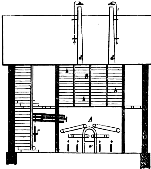
Fig. 362.—Section of seed-kiln.
